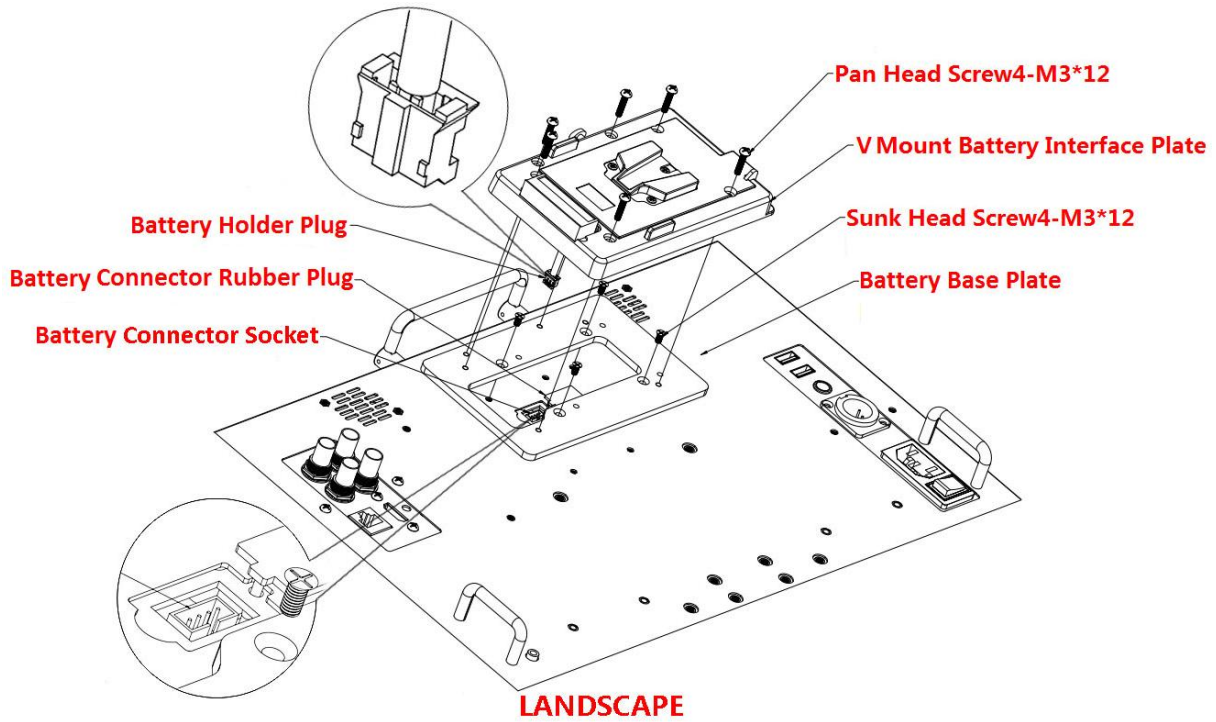
Figure 5.2-4 V-mount Battery Plate in Landscape
