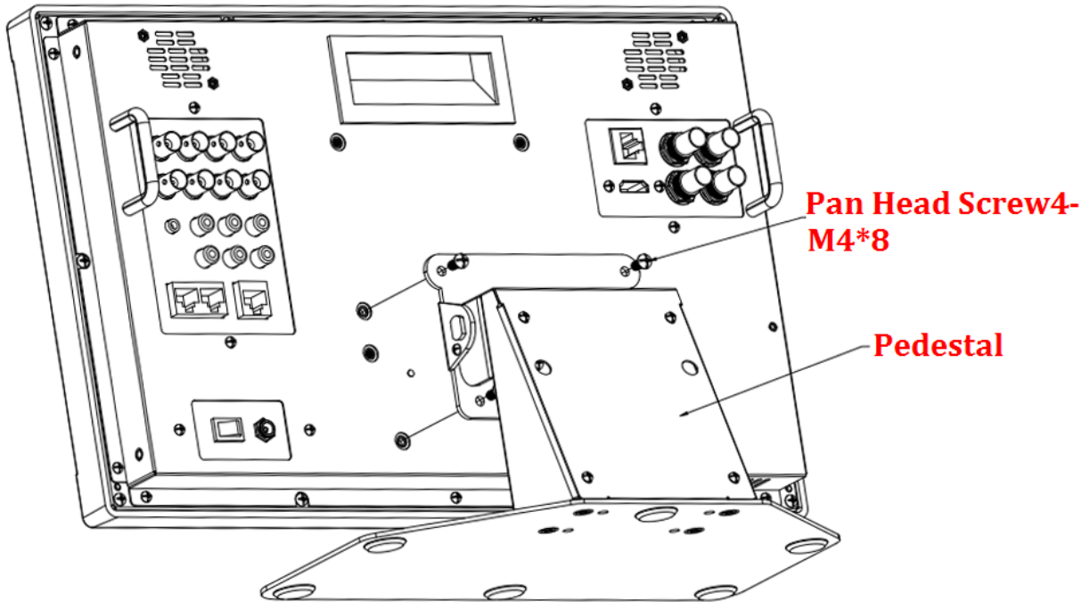
Figure 2-1 Assemble Pedestal of LCM156-E
