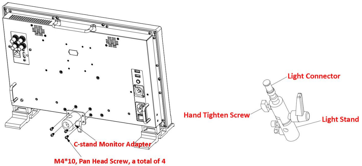
Figure 5.2-14 Adapter C-Stand to LCM-E Monitor
