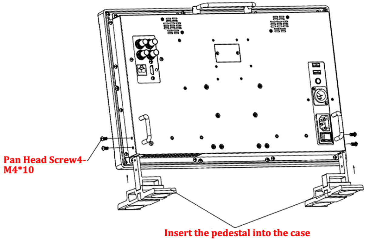
Figure 2-2 Assemble Pedestal of LCM170-E
