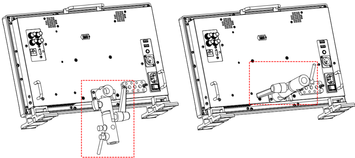
Figure 5.2-15 Connecting to Light Stand
