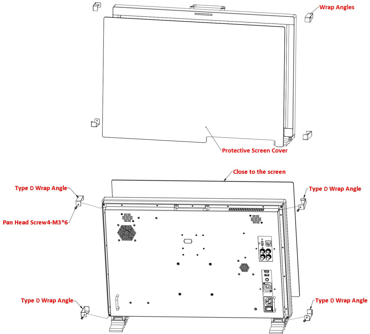
Figure 5.2-13 Mount a Protective Screen for LCM240-E
