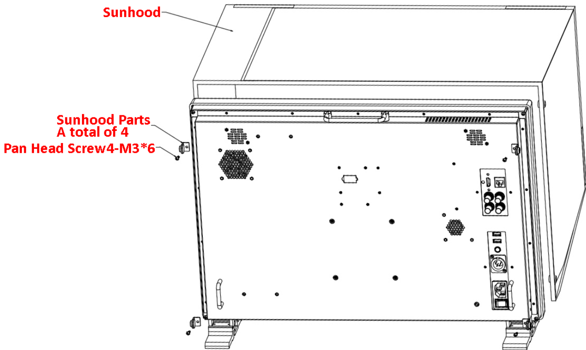
Figure 5.2-9 Mount a Sunhood for LCM240-E
