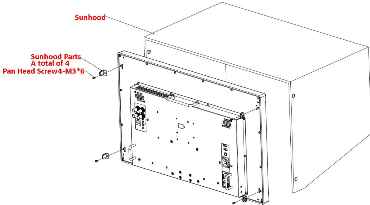
Figure 5.2-8 Mount a Sunhood for LCM230-E
