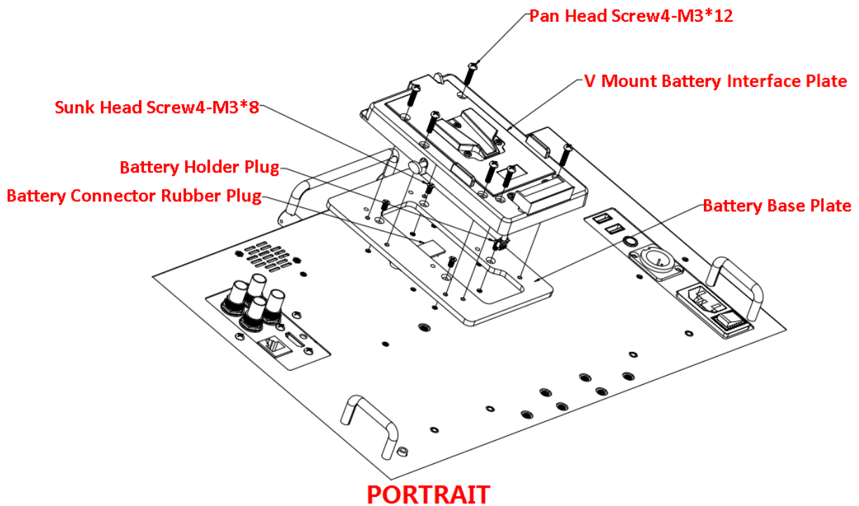
Figure 5.2-5 V-mount Battery Plate in Portrait
