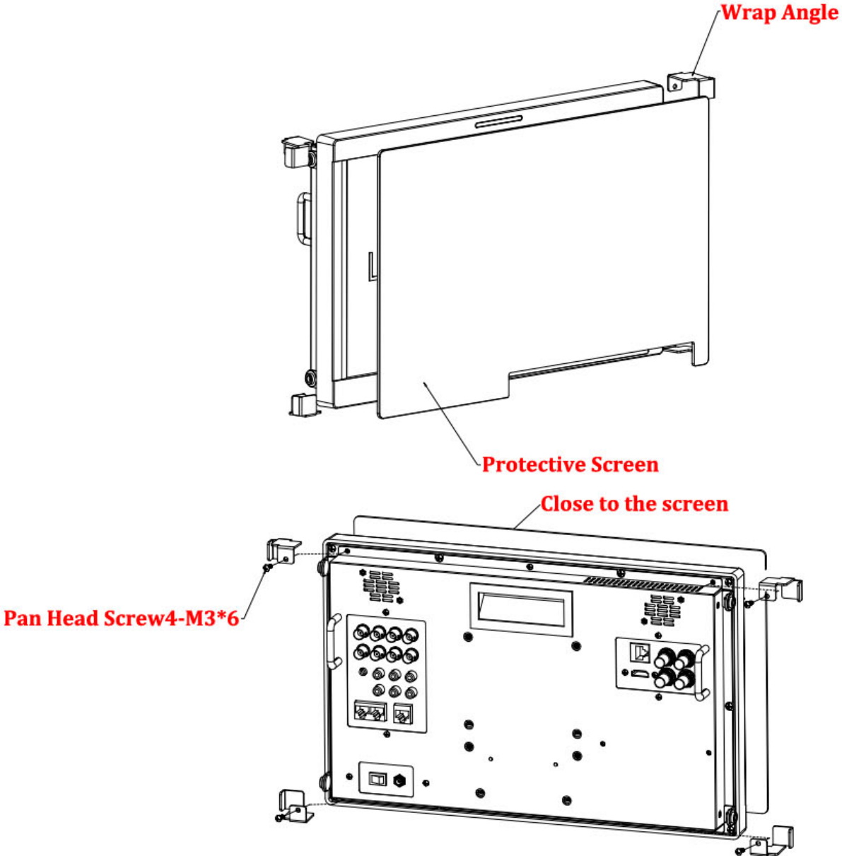
Figure 5.2-10 Mount a Protective Screen for LCM156-E
