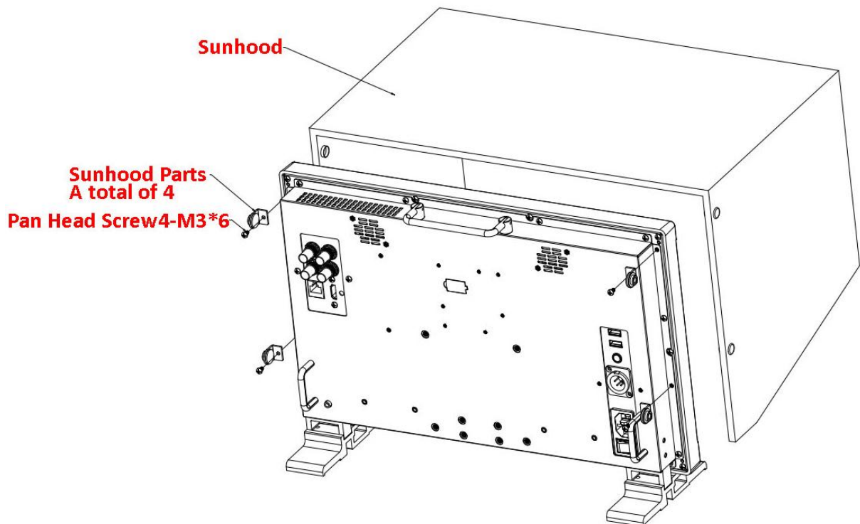
Figure 5.2-7 Mount a Sunhood for LCM170-E/LCM215-E
