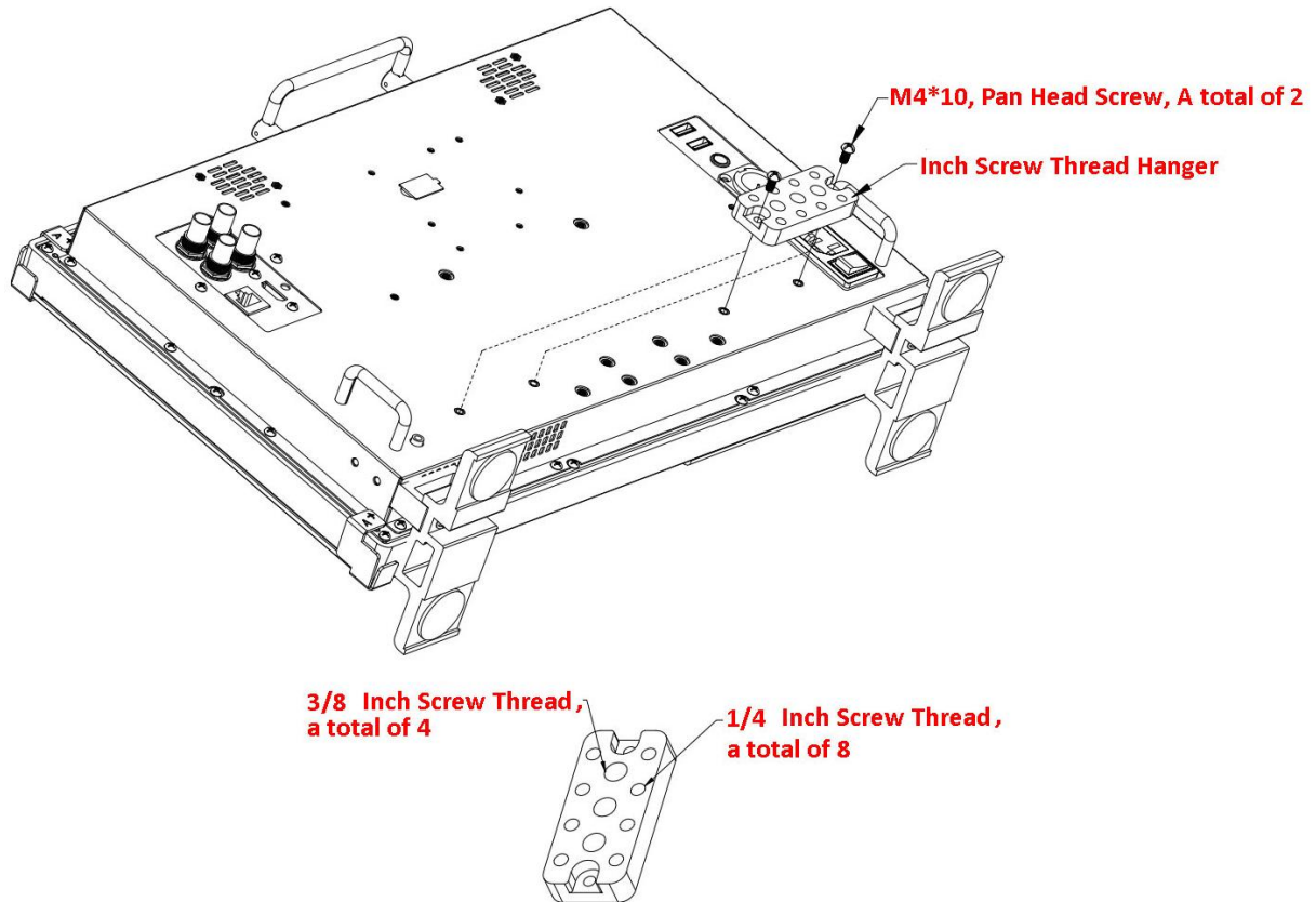
Figure 5.2-16 Inch Screw Thread Hanger
