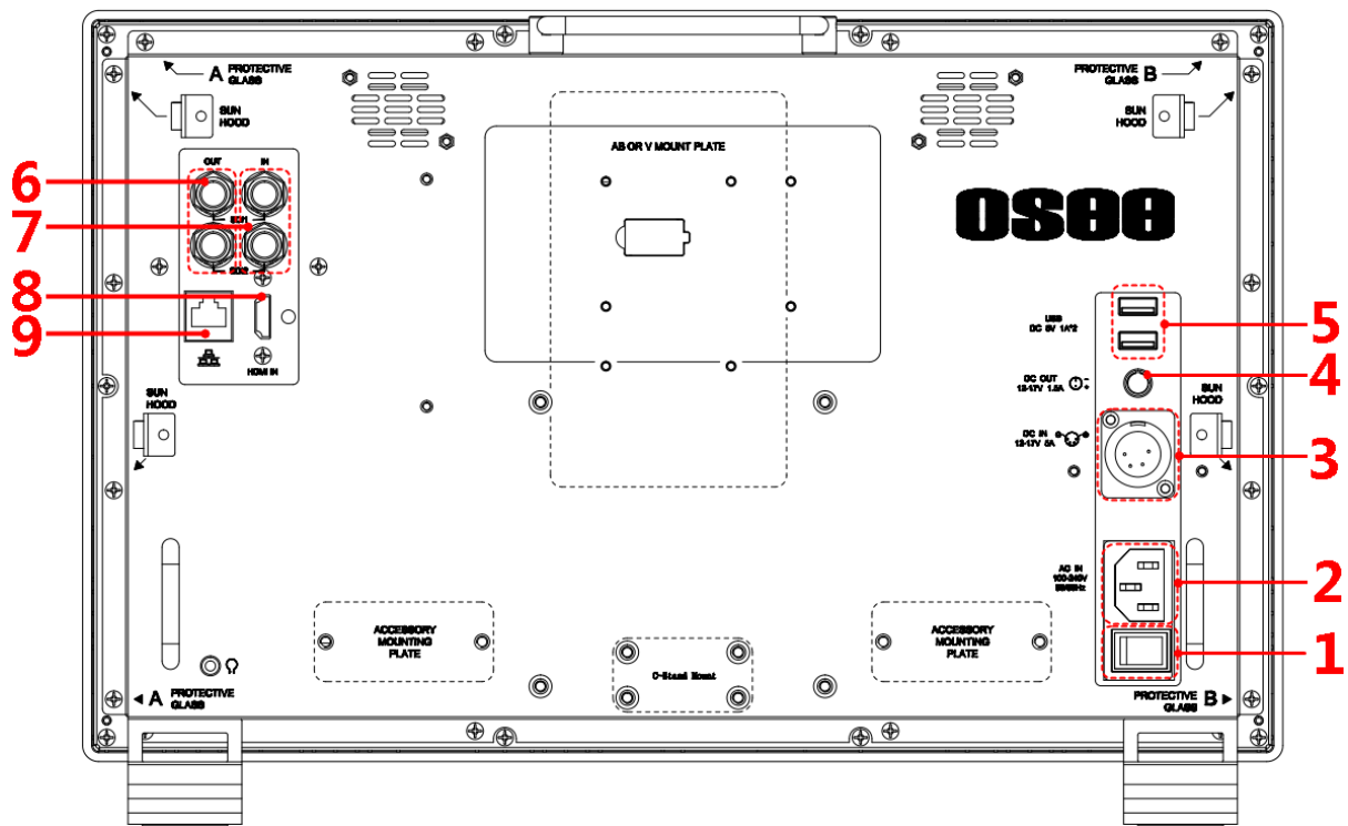
Figure 3.2-3 The Rear Panel of LCM170-E Monitor
