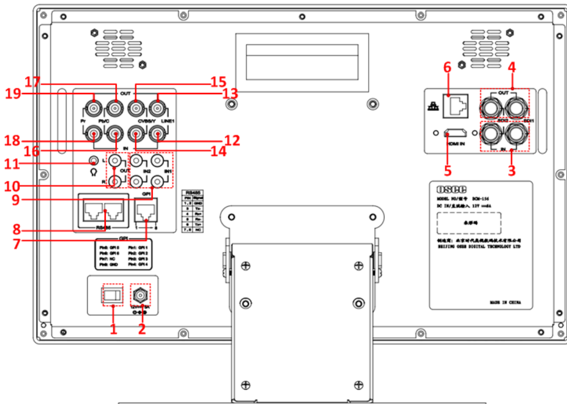
Figure 3.2-1 The Rear Panel of LCM156-E Monitor
