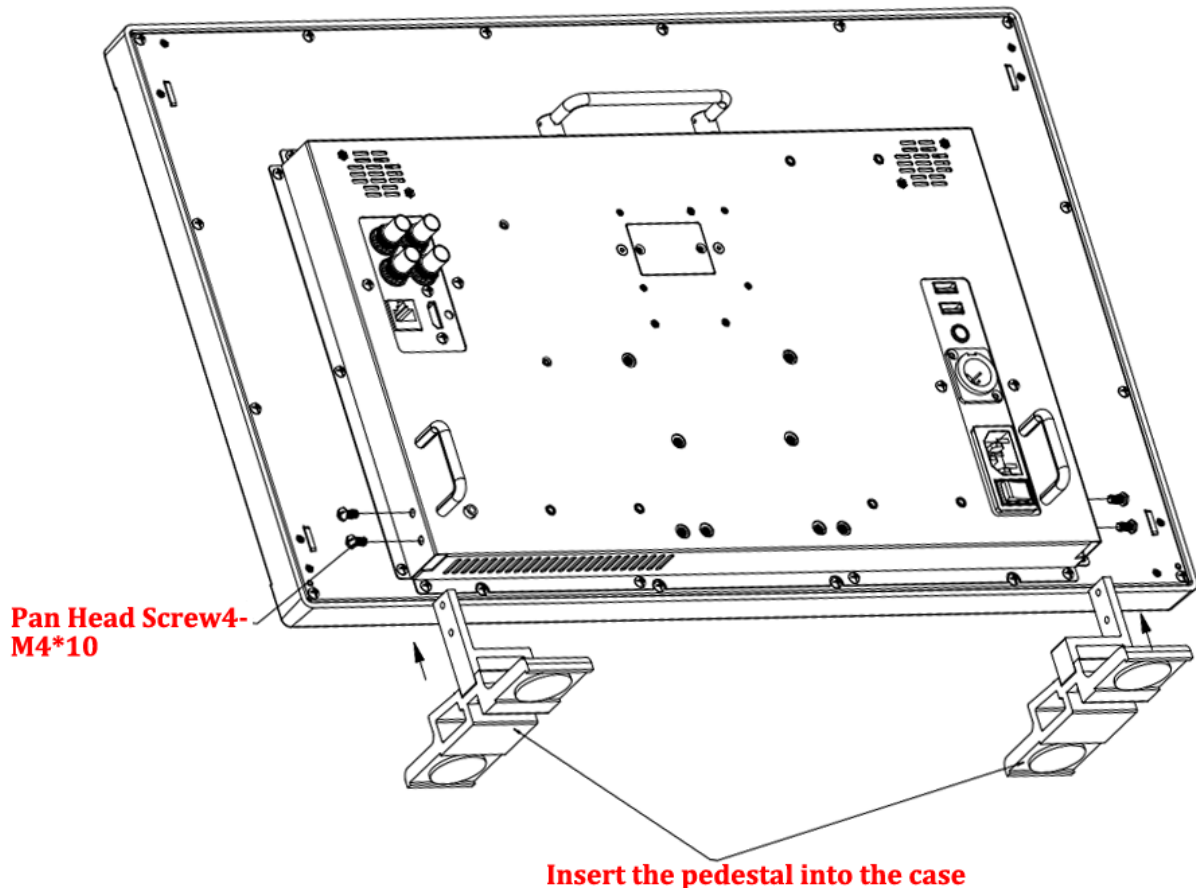
Figure 2-3 Assemble Pedestal of LCM230-E
