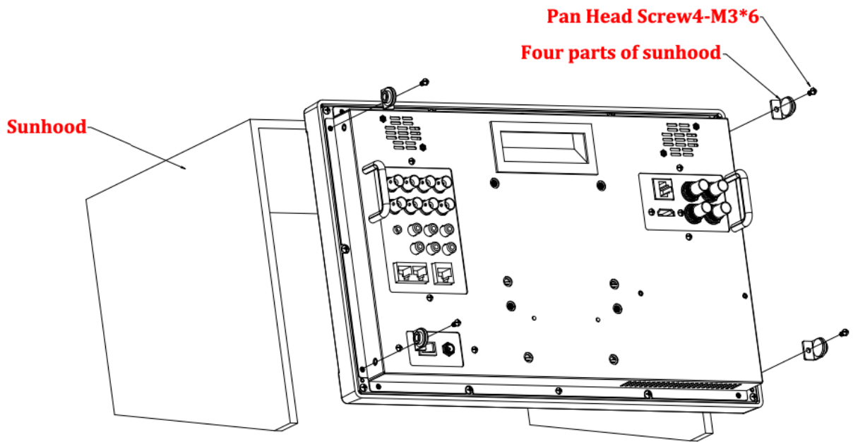
Figure 5.2-6 Mount a Sunhood for LCM156-E
