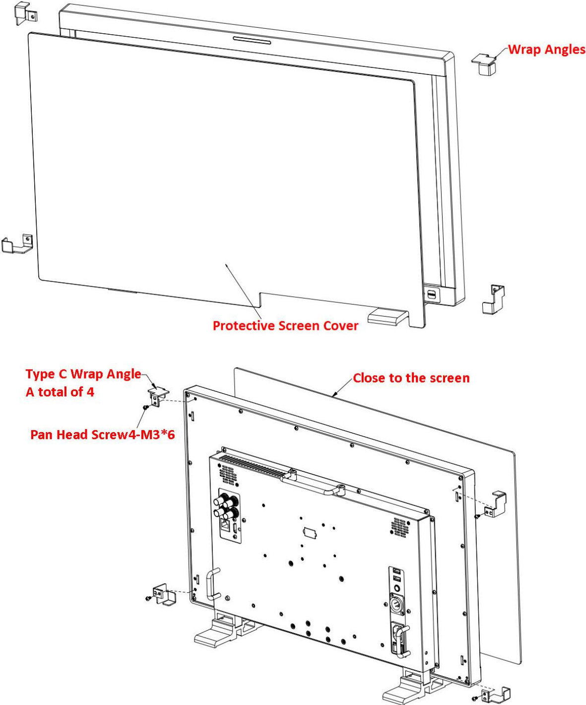
Figure 5.2-12 Mount a Protective Screen for LCM230-E
