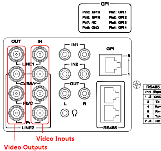
Figure 3.2-2 Video Input/Output Interfaces
