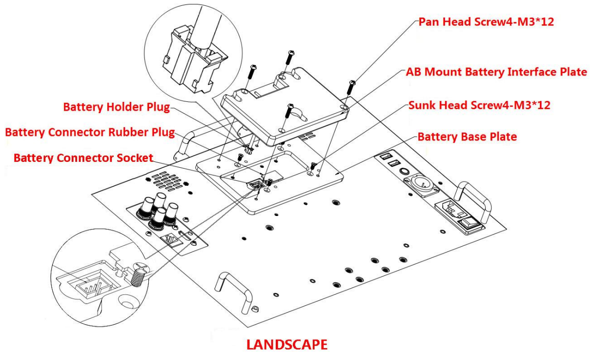
Figure 5.2-2 AB-mount Battery Plate in Landscape
