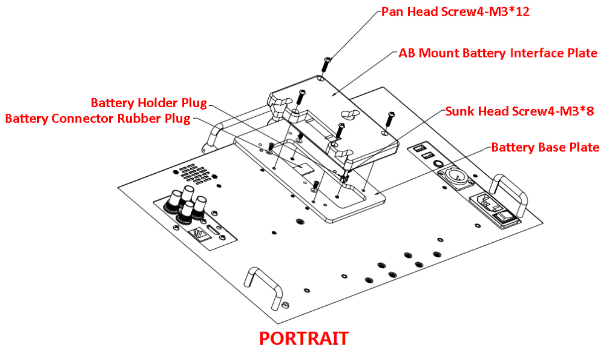
Figure 5.2-3 AB-mount Battery Plate in Portrait
