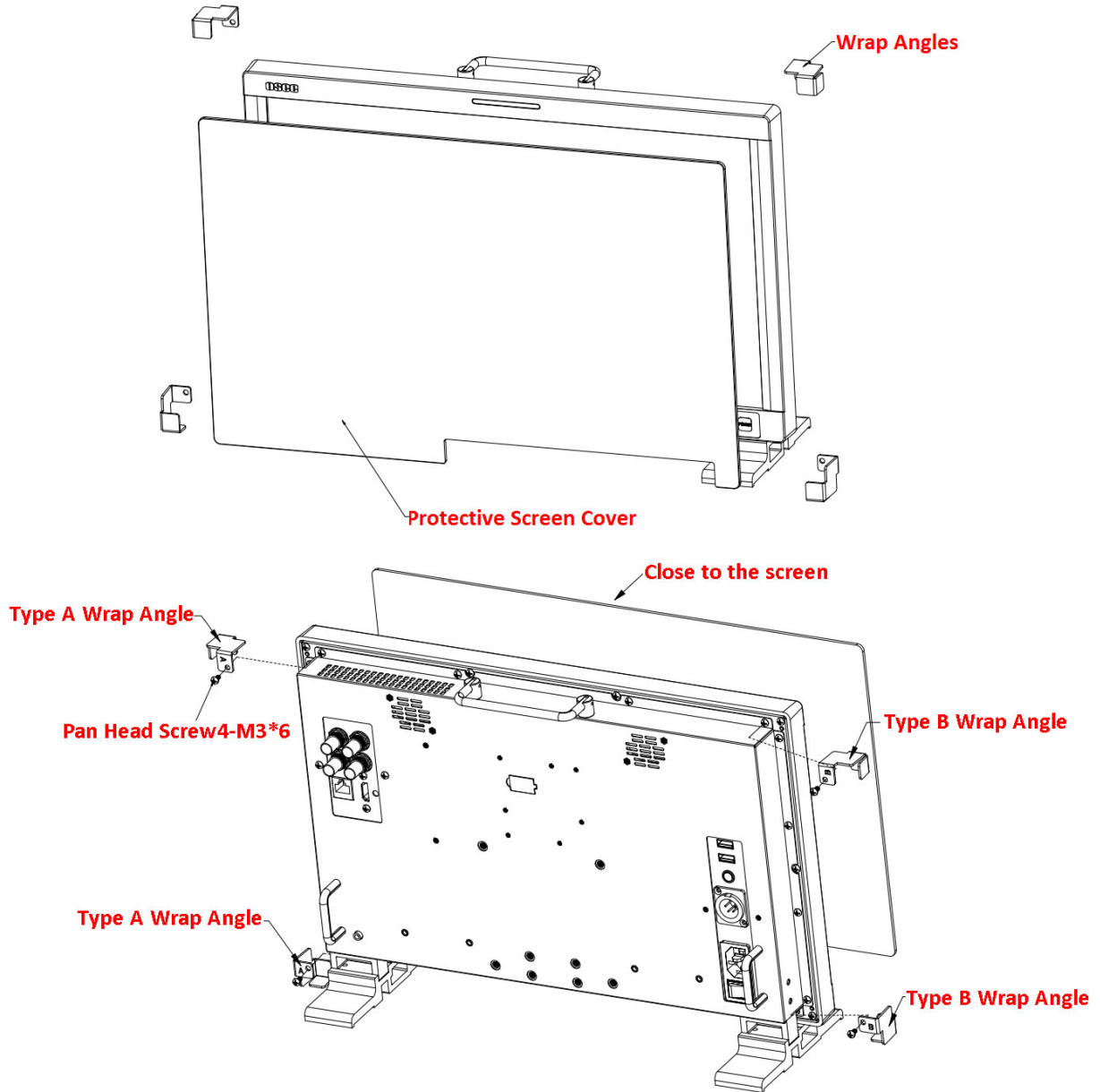
Figure 5.2-11 Mount a Protective Screen for LCM170-E/ LCM215-E
