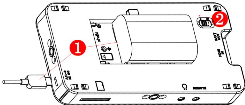
Figure 4.4-1 Power Switch
