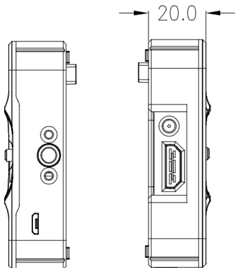
Figure 7.2-3 Side View(Unit: mm)
