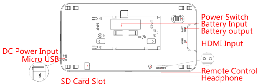
Figure 4.1-1 Parts in Rear Panel
