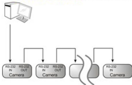
■ RS-232 pins definition instructions
