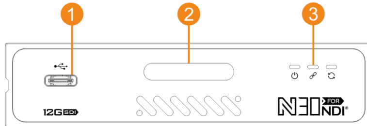
1.TYPE-C expansion port 2.Tally 3.Working indicator
